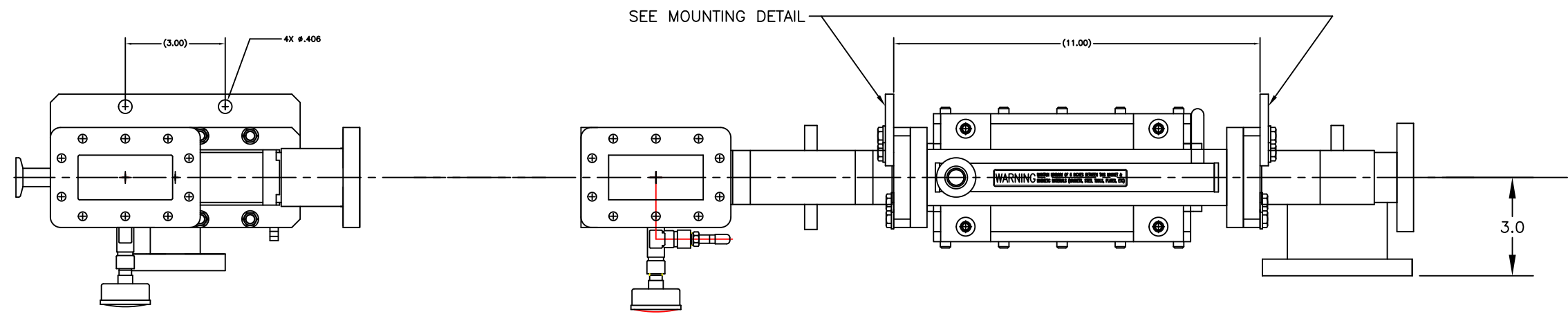
MOUNTING DETAIL
